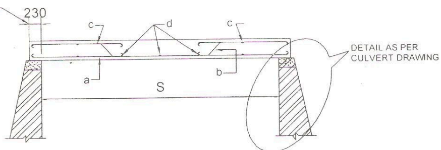
DETAILS OF DESIGN FOR SLAB CULVERT
