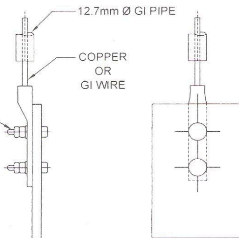
ENLARGED DETAIL-A
