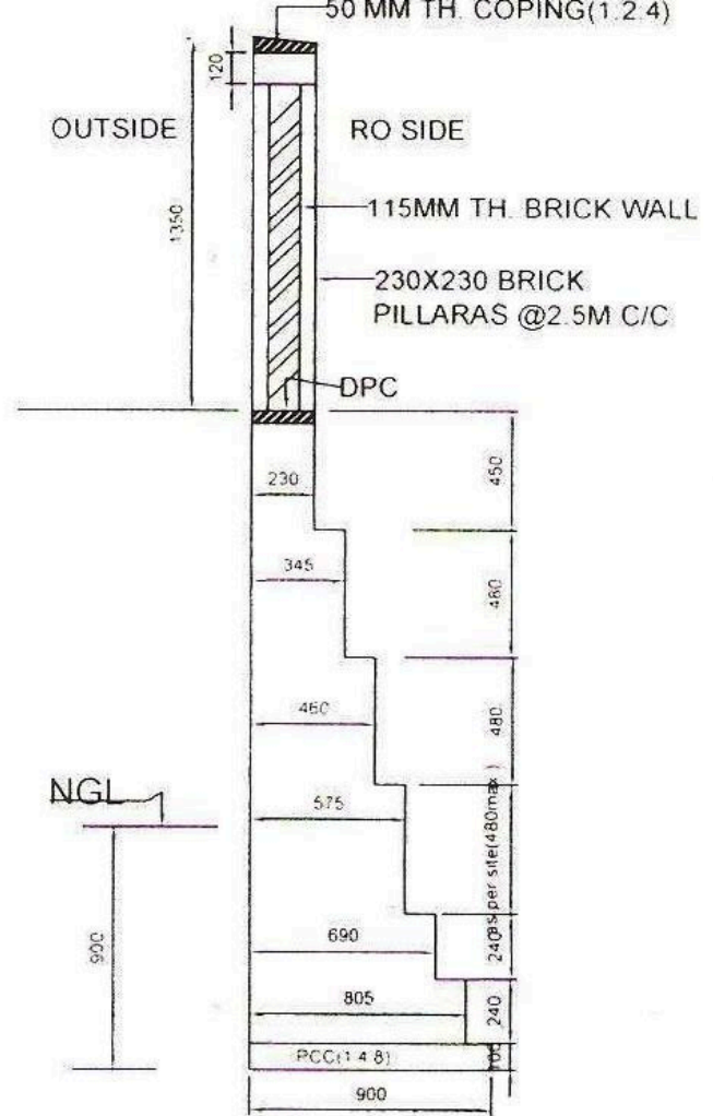
SECTION OF COMPOUND WALL (FILLING UPTO 1800MM)
