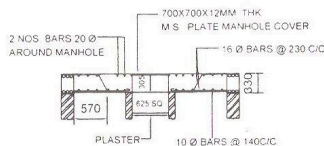
CROSS SECTION THROUGH MANHOLE
