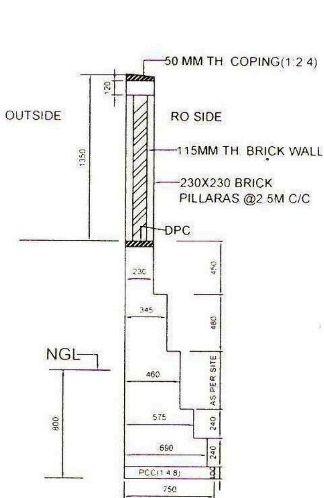
SECTION OF COMPOUND WALL (FILLING UPTO 1200MM)
