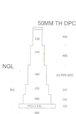
SECTION OF SALES BUILDING FOUNDATON(FILLING UPTO 1200MM)
