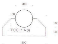
LAYING OF HUME PIPE
