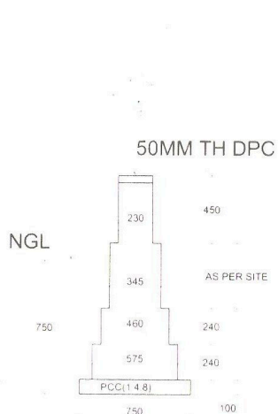
SECTION OF SALES BUILDING FOUNDATON(FILLING UP TO 600MM)
