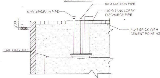
DETAILS AT 'C' (FERER DTAIL DRG NO RE 382)
