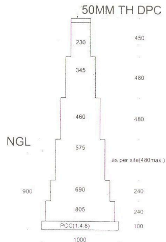
SECTION OF SALES BUILDING FOUNDATON(FILLING UPTO 1800MM)
