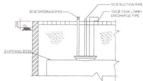
DETAILS AT 'C' (REFER DETAIL DRG NO RE 382)
