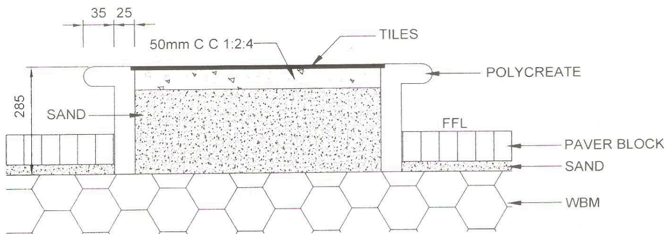
SECTION AT Y-Y
