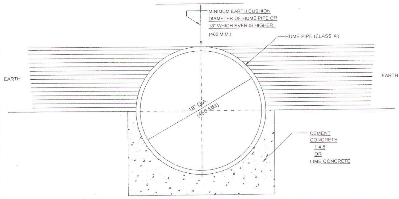
DETAILS OF HUME PIPE FOUNDATION
