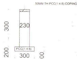
SECTION OF KERB WALL FOR TANKS
