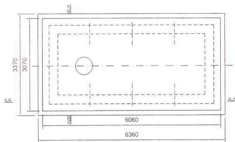
TANK IN MASONRY PIT WITH R.C.C. SLAB ON TOP
