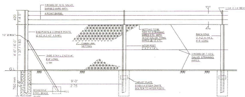
CHAIN LINK FENCING
