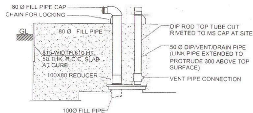
DETAILS AT 'C'
