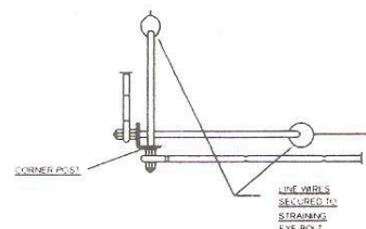
METHOD OF SECURING LINE WIRES TO POSTS
