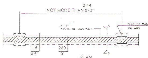
BRICK MASONRY COMPOUND WALL
