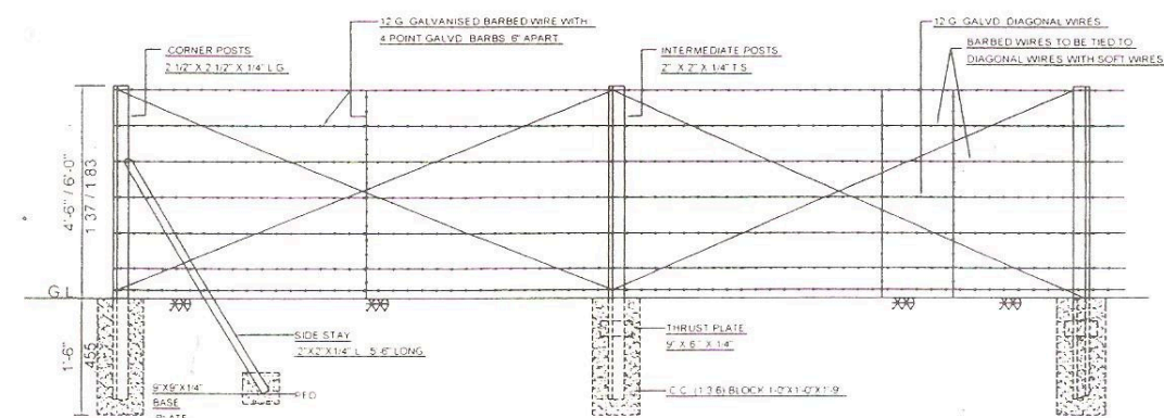
BARBED WIRE FENCING
