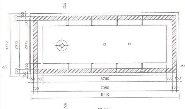
TANK IN MASONRY PIT
